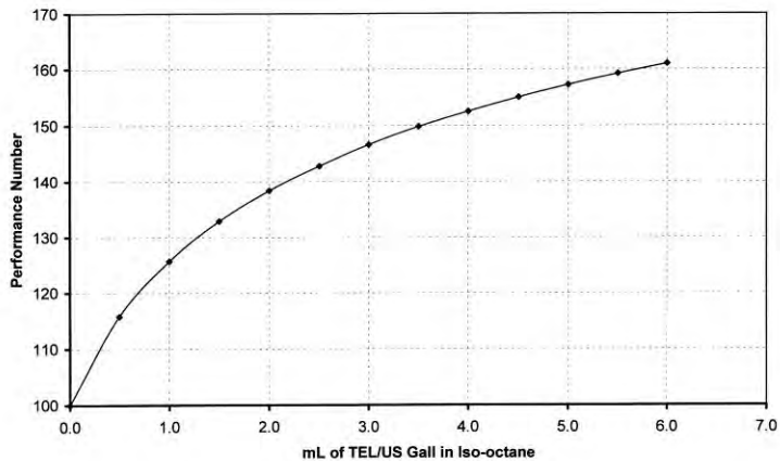
Figure 13. Relationship between Performance Numbers and Iso-octane plus TEL.
