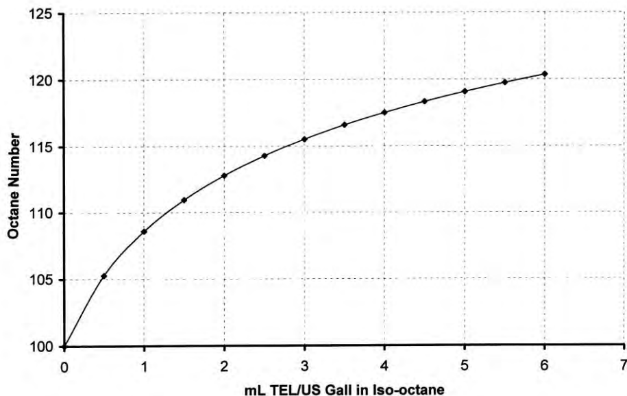
Figure 7. Octane Numbers above 100.
