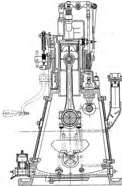
Figure 3. Variable Compression Ratio CFR Engine. 19
