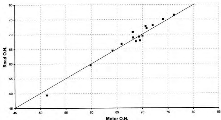
Figure 11. 1934 Correlation between Road and Laboratory Octane Numbers.
