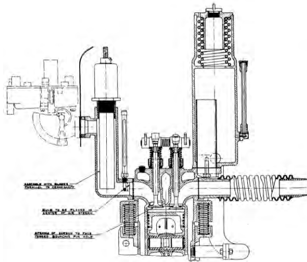
Figure 9. CFR Engine Modifications.
