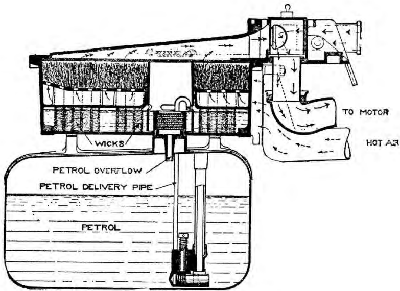
Figure 2. Lanchester Wick Carburettor.
