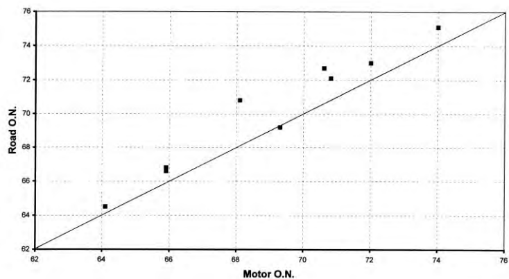
Figure 12. 1934 Correlation between Road and Laboratory Octane Numbers for non-Paraffinic Fuels
