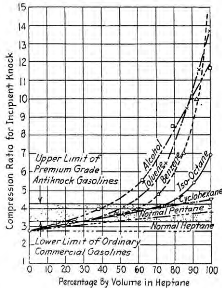
Figure 6. Detonation Characteristics of some Antiknock Standards.
