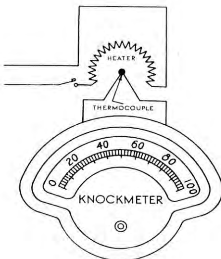
Figure 5. Modified Knockmeter. 22
