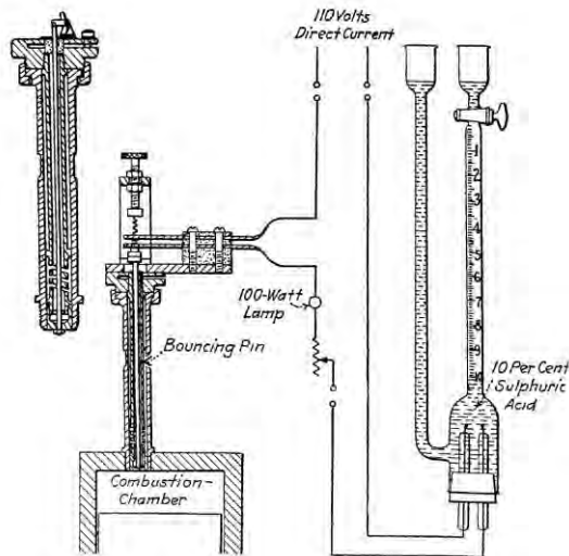
Figure 4. Original Bouncing Pin Knock Detection Equipment. 20
