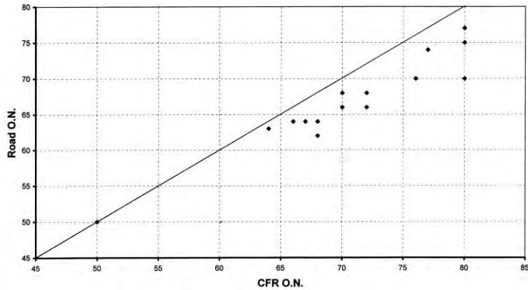
Figure 8. 1932 Correlation between Road and Laboratory Octane Numbers.
