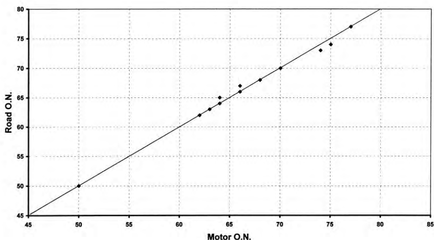
Figure 10. 1932 Correlation between Road and Laboratory Octane Numbers following Modifications to the Laboratory Engine and Test Procedure.
